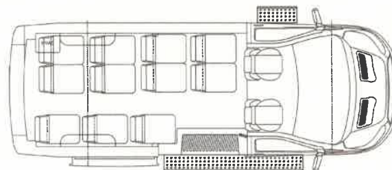
12-PASSENGER
