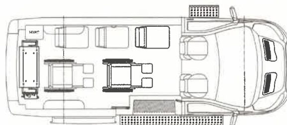
4-PASSENGER + 2-WHEELCHAIR
