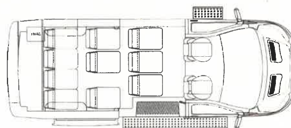
11-PASSENGER + REAR LUGGAGE
